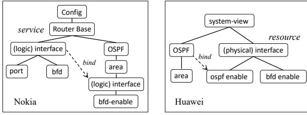
Fig. 2. Configuration logic graph for Fig. 1(c).
